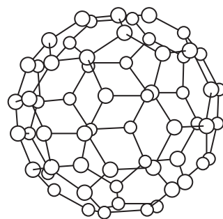
fullerene molecule
